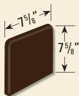
SURFACE BULLNOSE (SB8888)
