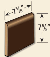
SURFACE BULLNOSE (SB888)
