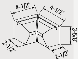
Rolok Sill Internal Corner
